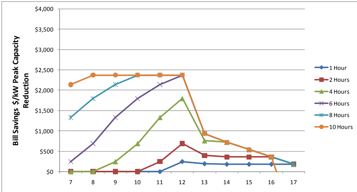
Figure 25: Broad Scenario Analysis – Bill Savings Sensitivity to Tech. Lifetime – 30 Year Lifetime
