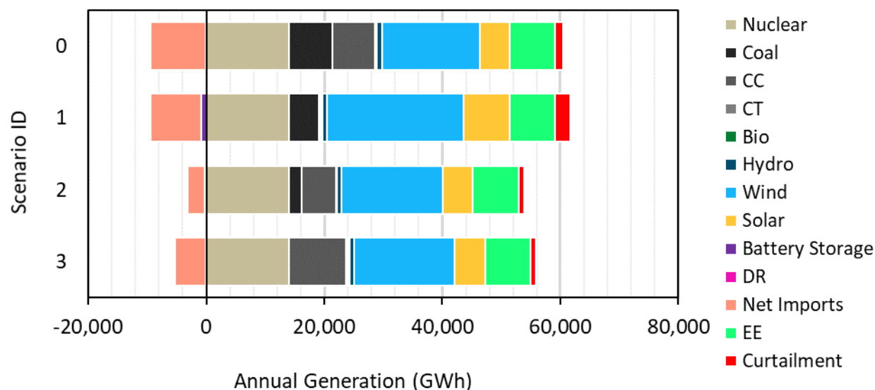
Figure 5-6. 2030 snapshot: annual generation (GWh) for Scenarios 1, 2 & 3
