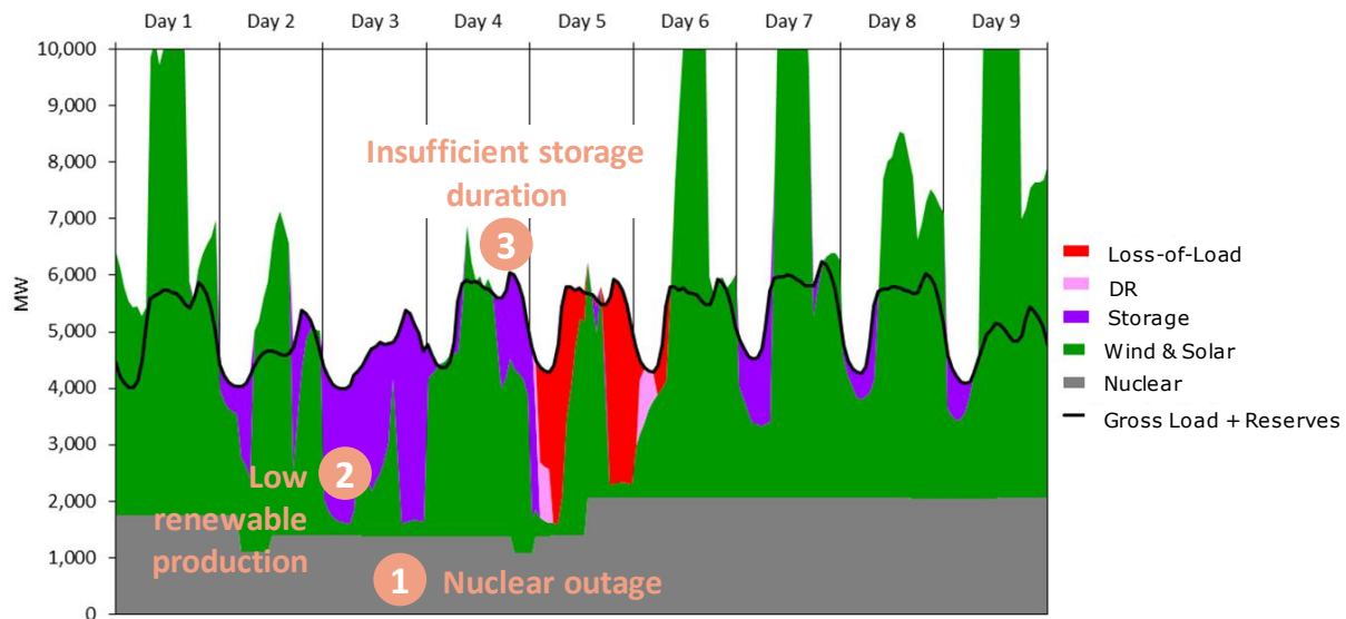
Figure 4-4. Illustrative sample of hourly dispatch patterns in a 100% Carbon Reduction Scenario
