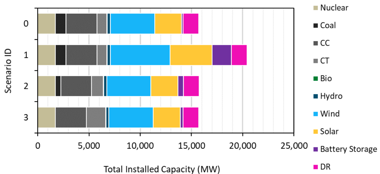
Figure 5-5. 2030 snapshot: installed capacity (MW) for Scenarios 1, 2 & 3
