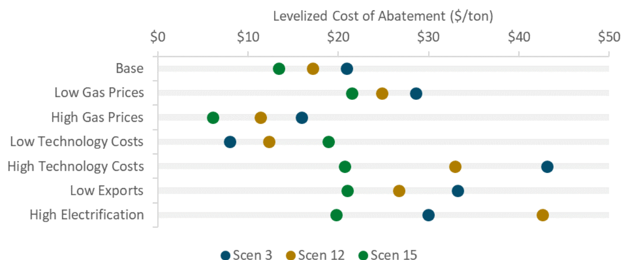
Figure 5-21. Sensitivity analysis on levelized cost of abatement across scenarios
