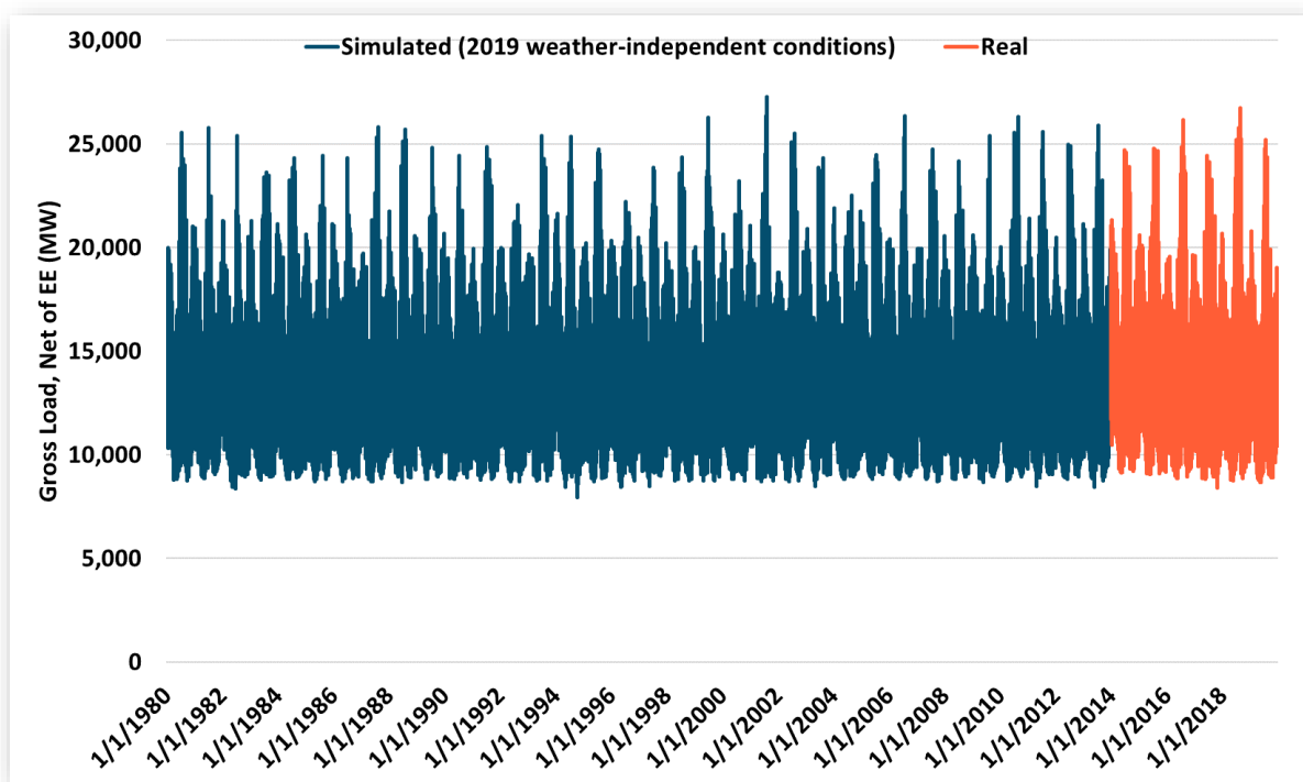
Figure 7-9. Real and Simulated New England System Load
