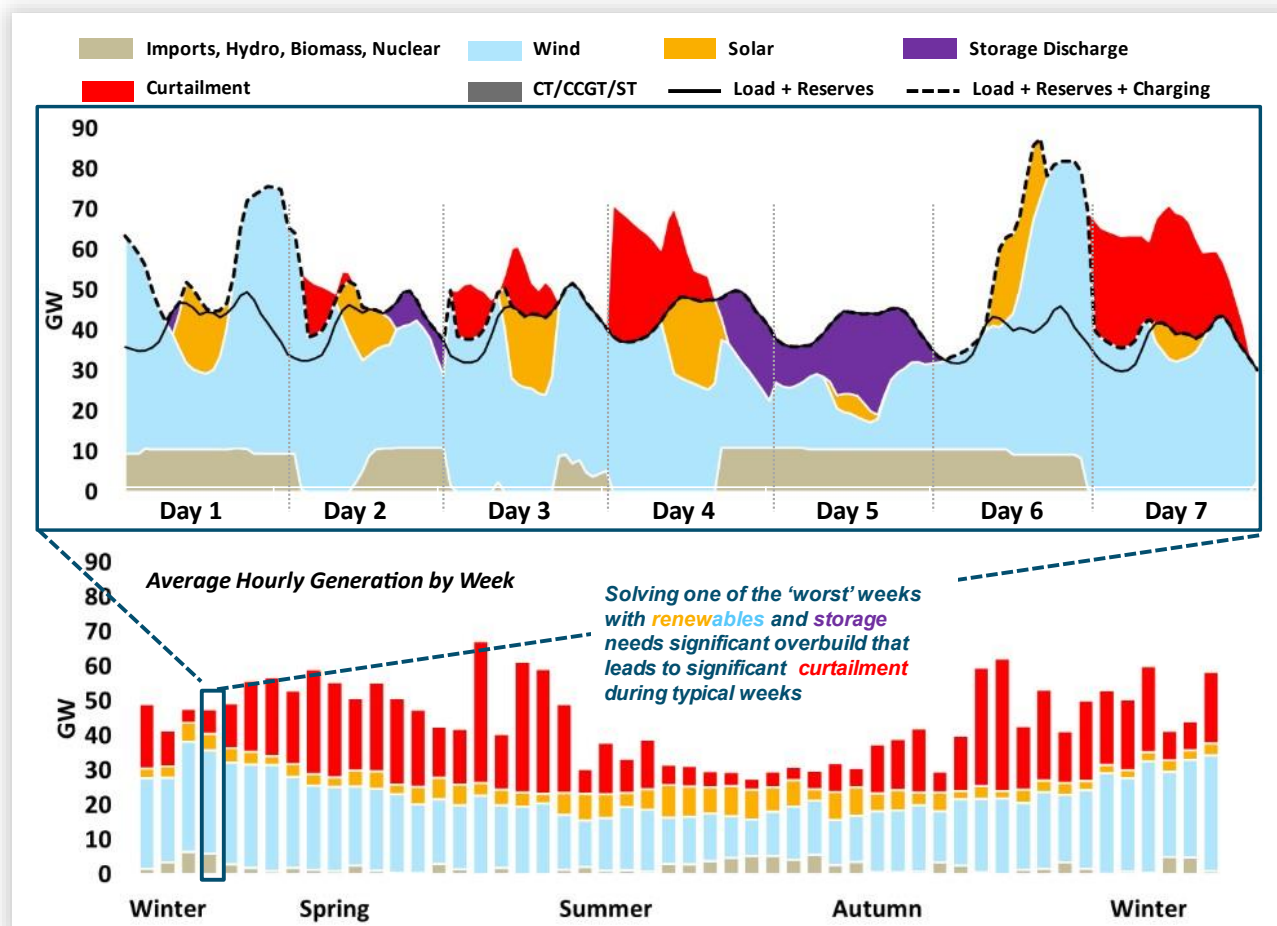
Figure 4-11. Illustrative Dispatch over a Critical Week in 2050 (No Combustion Resources with High Electrification Scenario)
