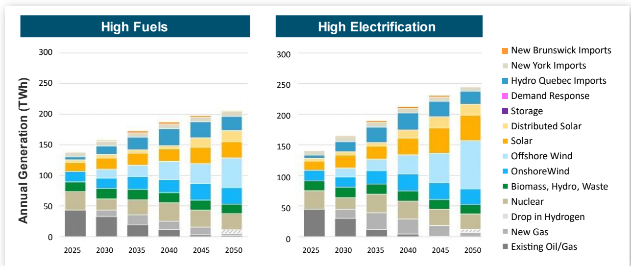
Figure 4-7. Total Electricity Generation
