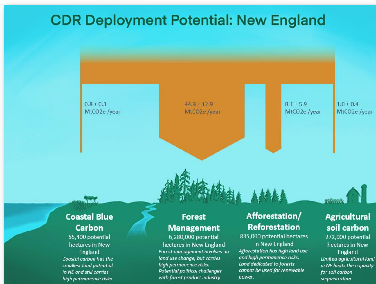
Figure 5-2. Ranges for Natural CDR Potential in New England
