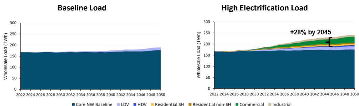
Figure 7. Annual energy load forecasts for Core Northwest
