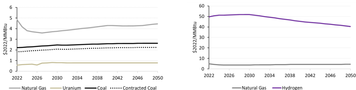
Figure 26. Fuel price forecasts for natural gas, coal, uranium, and hydrogen
